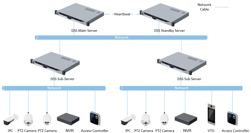
Figure 1-3 Hot standby
